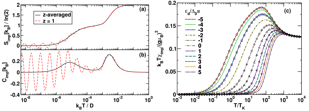
Fig. 6: Temperature dependence of, (a), the impurity entropy, S_{\text{imp}}(T) , and, (b), the impurity specific heat, C_{\text{imp}}(T) , for the symmetric Anderson model with U/\Delta_0 = 12 and \Delta_0 = 0.001D . The calculations are for \Lambda = 4 , without z -averaging [ n_z = 1 , z = 1 (dashed lines)], and with z -averaging [ n_z = 2 , z = 1/4, 3/4 (solid lines)]. For \Lambda = 4 two z values suffice to eliminate the discretization oscillations [37]. (c) Impurity susceptibility, \chi_{\text{imp}}(T) , vs T/T_K for the asymmetric Anderson model with same parameters as above and several values of \varepsilon_d/\Delta_0 with T_K for symmetric model. Broken lines: FDM approach. Solid lines: conventional approach. Symbols: Bethe ansatz (for selected values of \varepsilon_d/\Delta_0 = -5, -3, -1, 0, +1, +3 ). NRG parameters: \Lambda = 10 with z -averaging [ n_z = 4 , z = 1/8, 1/2, 3/8, 3/4 ] [38]
