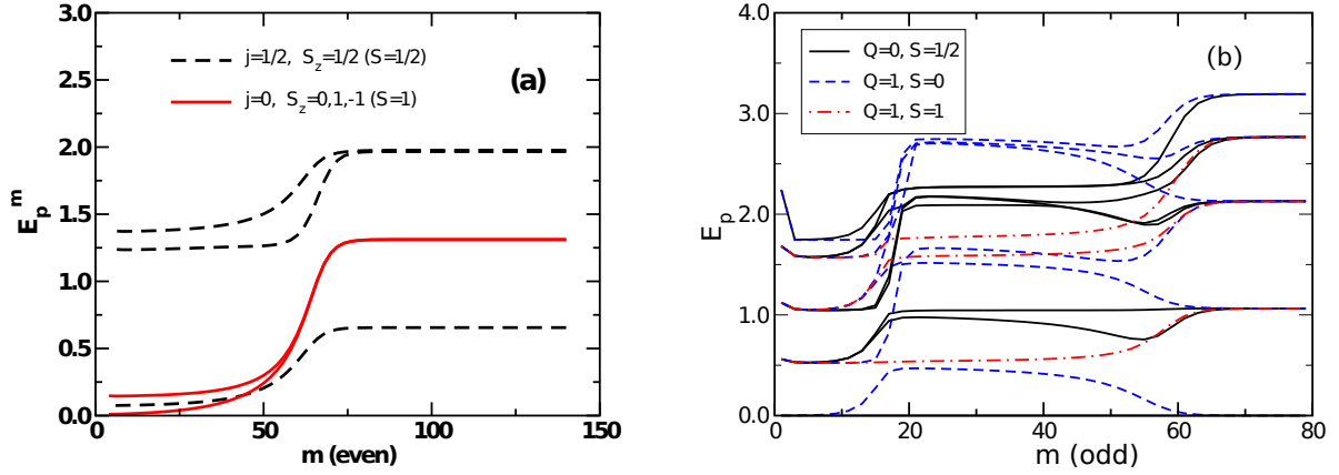
Fig. 5: (a) The lowest rescaled energy levels of the AKM for J_{\parallel} = 0.443 and J_{\perp} = 0.01 . The states are labeled by conserved pseudospin j and total S_z (adapted from [30]). (b) The flow of the lowest many-body energy levels of the Anderson model for \varepsilon_d = -U/2 , U/\pi\Delta_0 = 12.66 , and \Lambda = 2.5 . States are labeled by quantum numbers for total charge Q and total spin S (adapted from [4, 2]).
